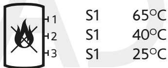
Program 4 Thermostat function Switch on sensor S1 Switch off sensor S3
